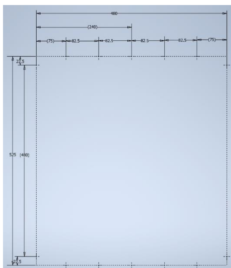
VRG20_40 (480x480/525)
