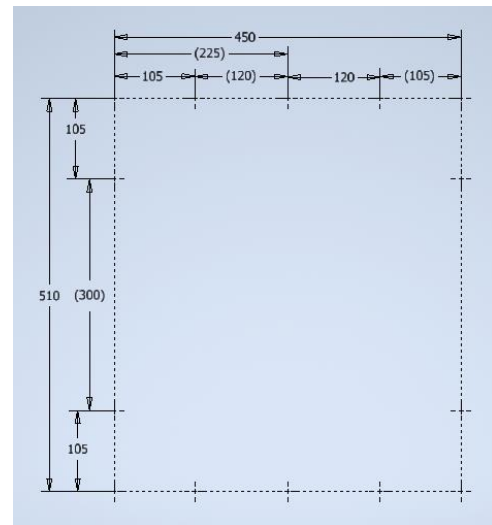
AB3000_AB4000_G65_G66 (450x510)
