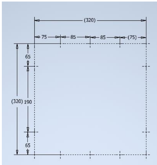
SBC410 (320x320)
