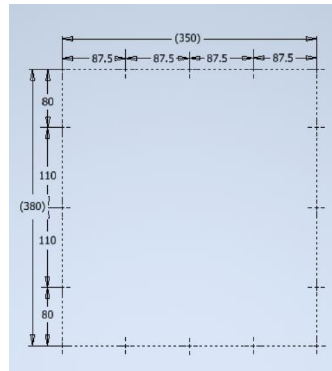
SB300_SBC610_SBC650 (350x380)
