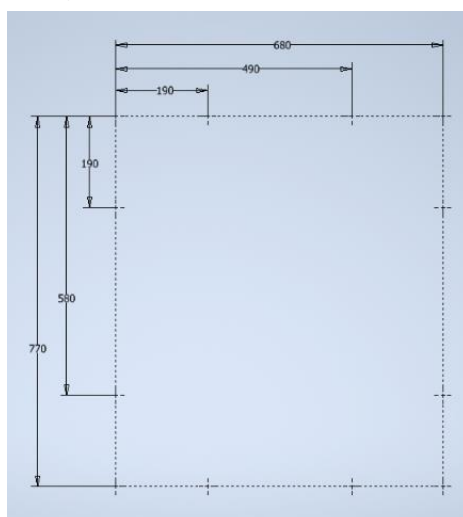
HB3100_HB3600_HB4100_HB4700 Ø39
