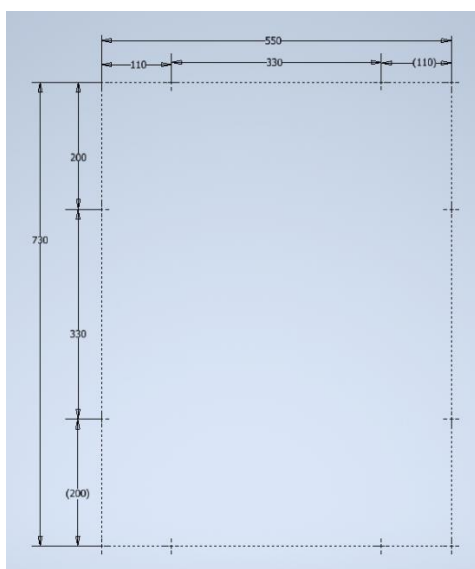
MSP1000R_1300R (550x730)
